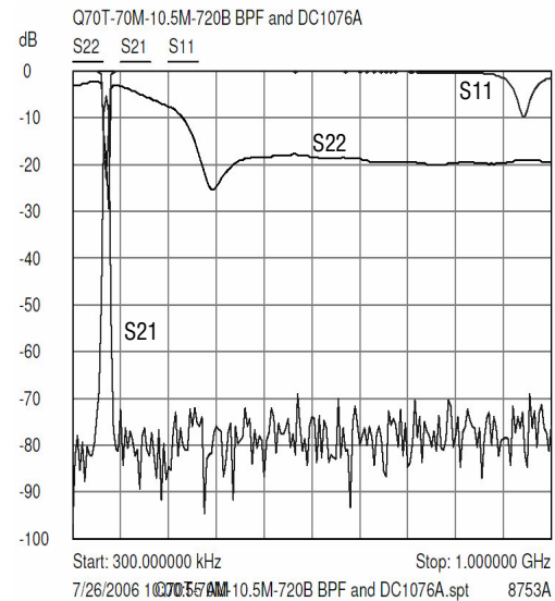
Figure 5. Cascaded filters.
