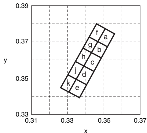
Fig. 7 Chromaticity Diagram
