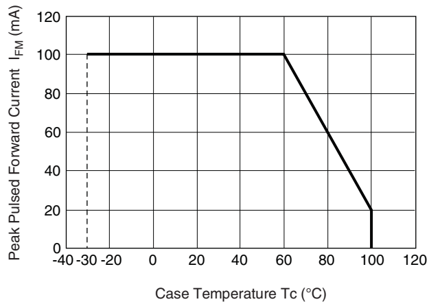
Fig. 3 Peak Pulsed Forward Current vs. Case Temperature
