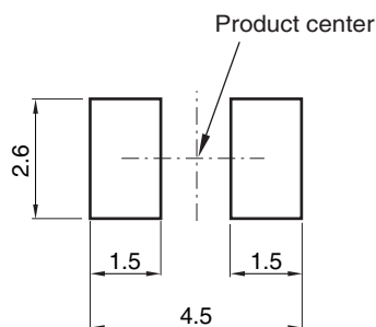
Fig. 16 Recommended Solder Pad Design
