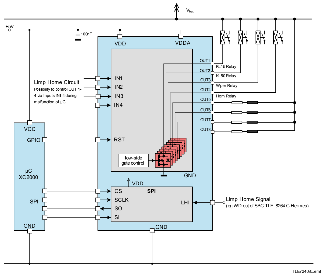
Figure 13 Application Diagram
