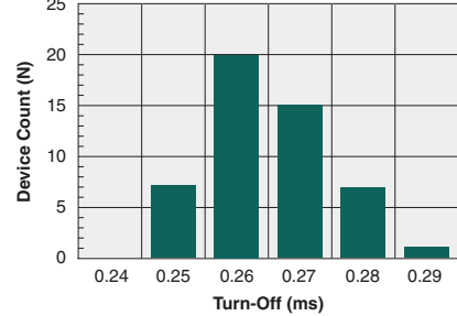
Typical Turn-Off Time ( N=50 , I_F=20\text{mA} , I_L=1A_{DC} )
