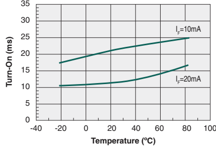
Typical Turn-On Time vs. Temperature ( I_L=1A_{DC} )
