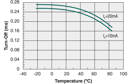
Typical Turn-Off Time vs. Temperature ( I_L=1A_{DC} )
