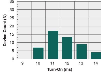
Typical Turn-On Time ( N=50 , I_F=20\text{mA} , I_L=1A_{DC} )
