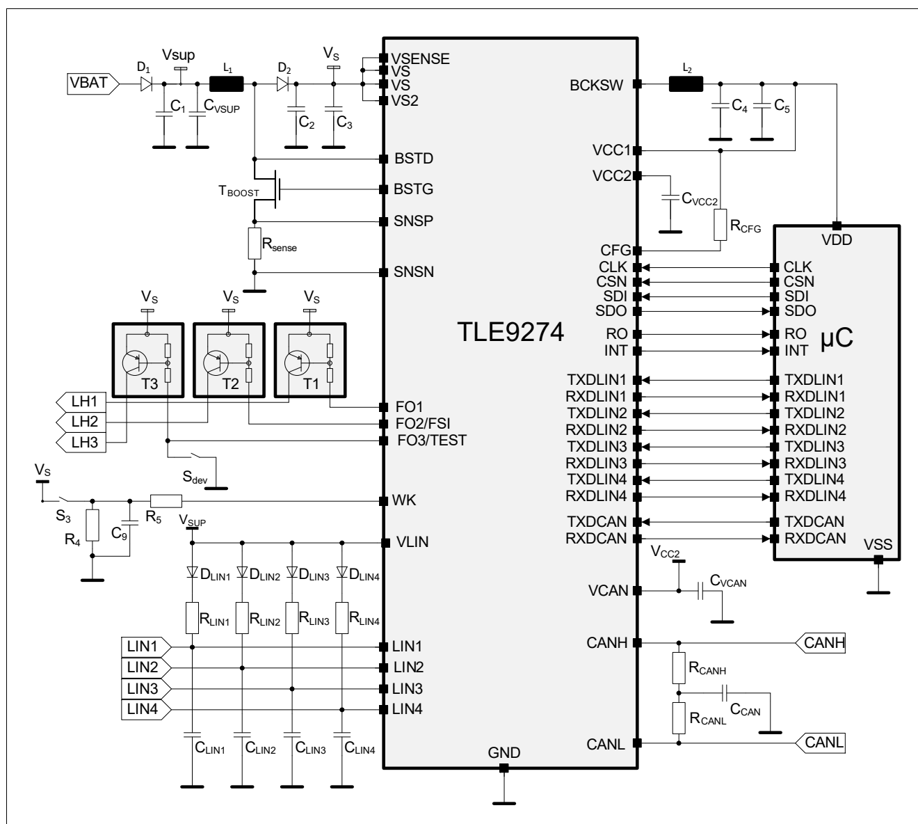
Figure 51 Application diagram
