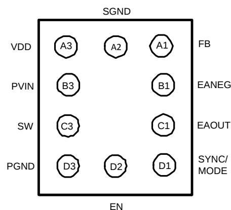
Figure 5. YPA Package Bottom View
