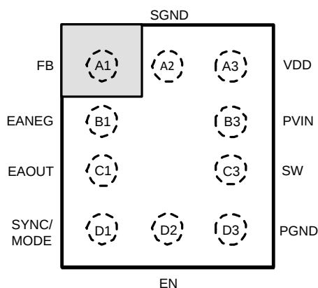
Figure 4. YPA Package Top View
