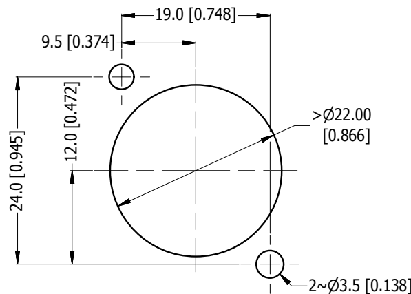
PANEL CUT OUT (SCALE 2:1)
