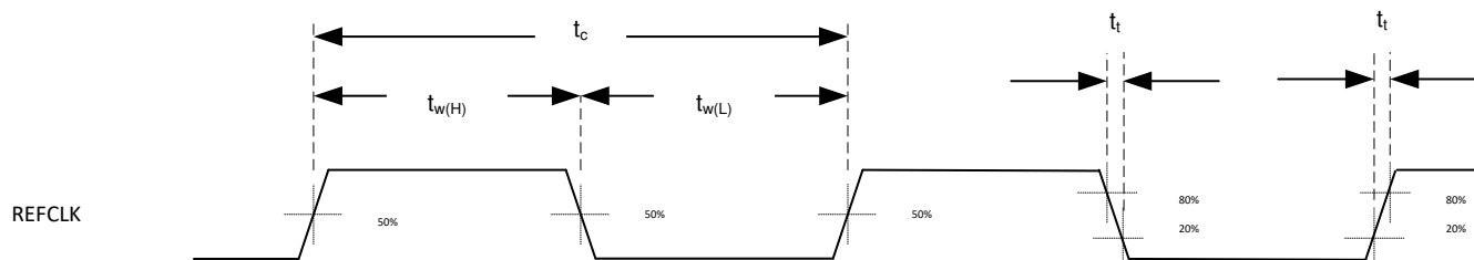
Figure 6-4. System Oscillators
