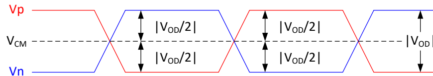
Figure 6-2. DMD Low-Speed Differential Voltage Parameters
