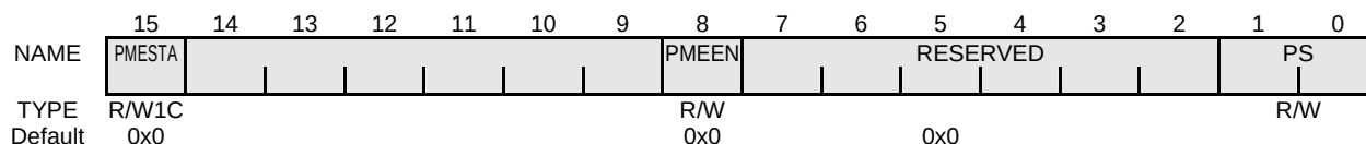
Figure 16-80 PMCSR Register
