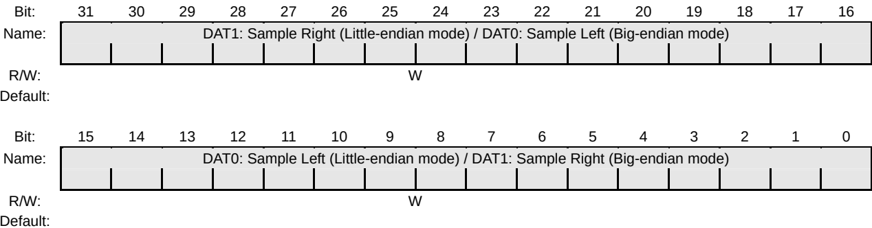
Figure 24-21 ACAUDODAT/ACSURRDAT Register
