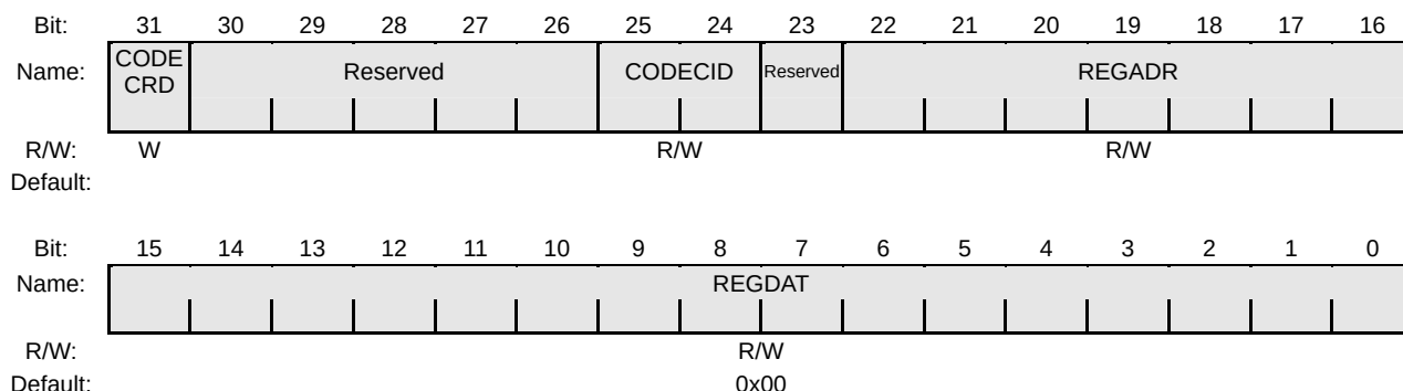
Figure 24-11 ACREGACC
