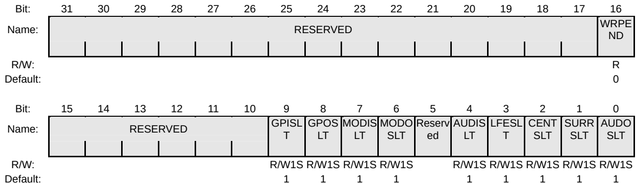
Figure 24-16 ACSLTEN Register
