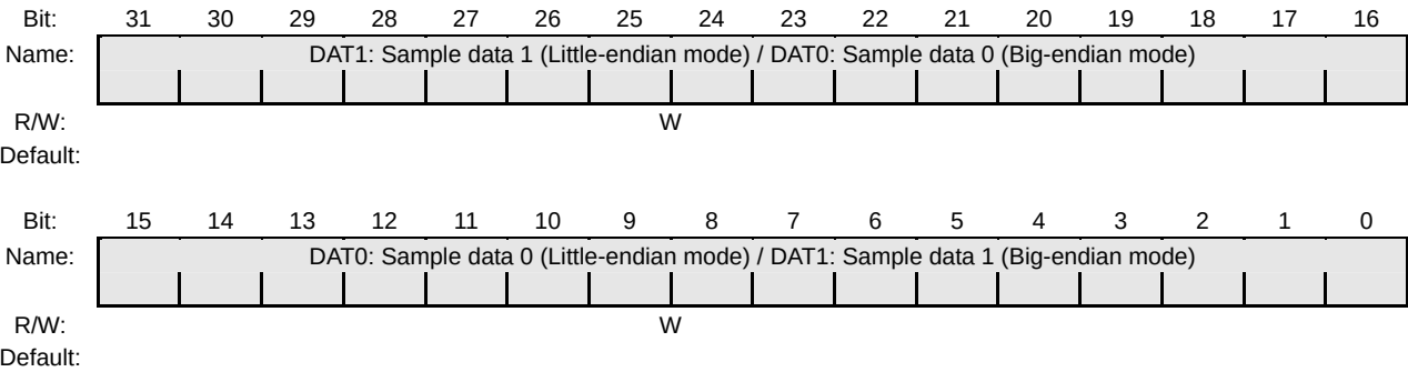
Figure 24-22 ACCENDAT/ACLFEDAT/ACMODODAT Register
