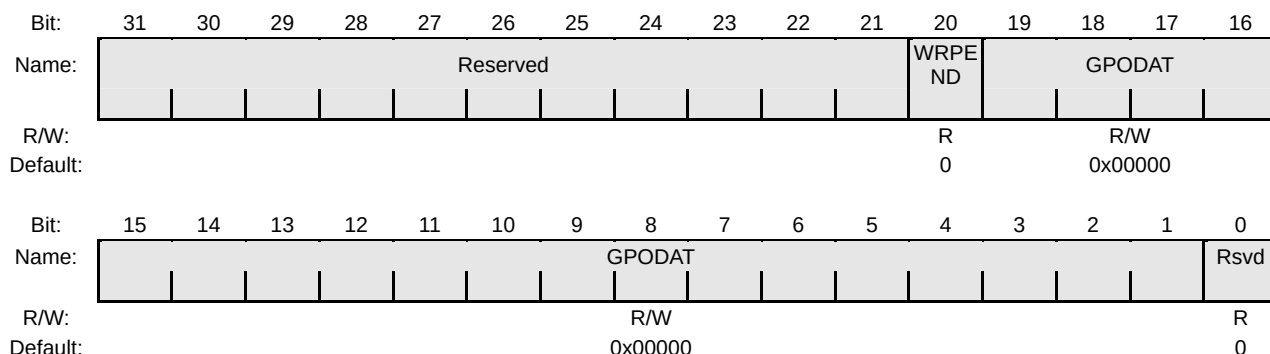
Figure 24-15 ACGPODAT Register
