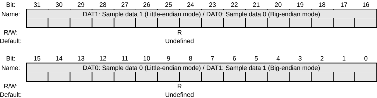
Figure 24-24 ACMODIDAT Register
