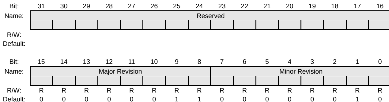
Figure 24-25 ACREVID Register
