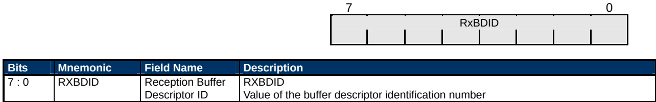
Figure 18-9 BDStat Field
