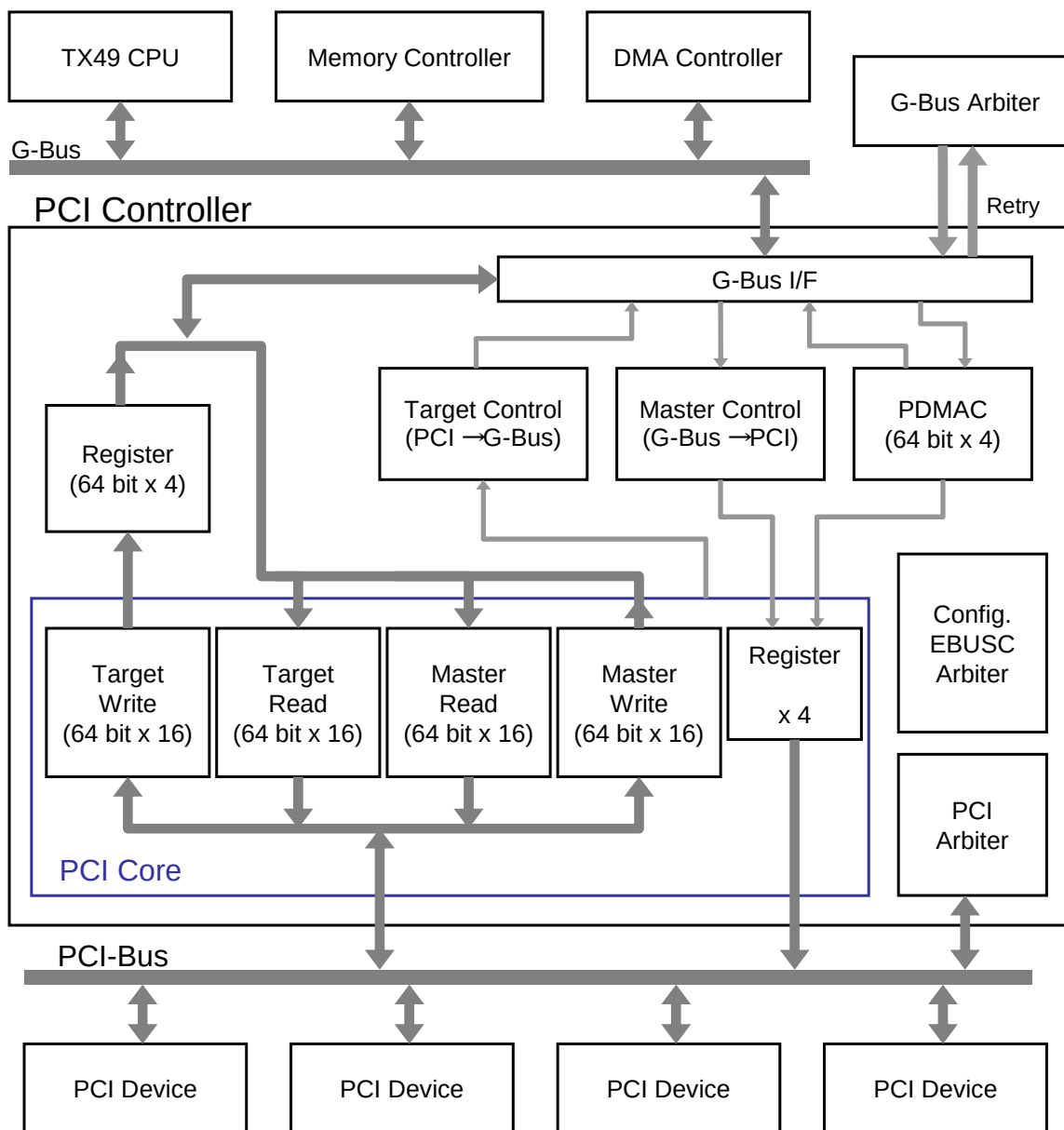
Figure 16-1 PCI Controller Block Diagram
