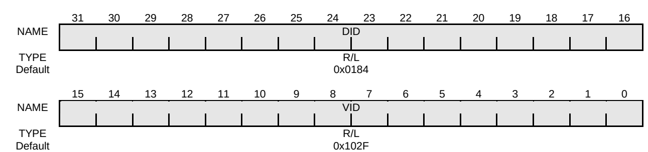
Figure 16-14 ID Registers
