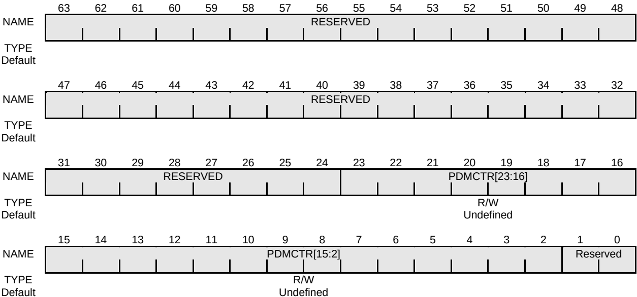
Figure 16-71 Count Register
