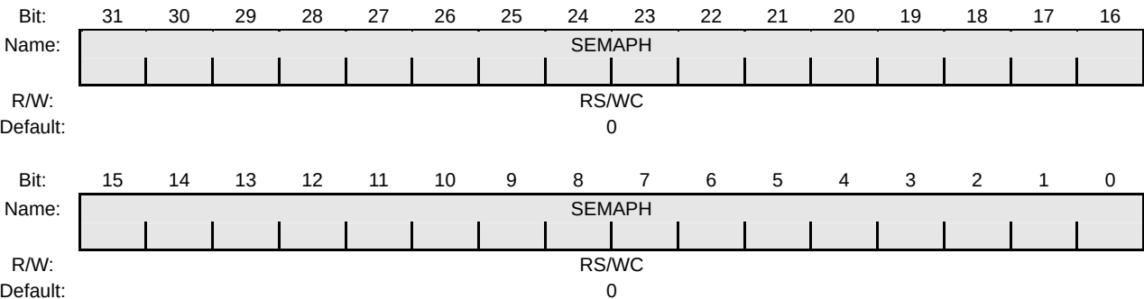
Figure 24-13 ACSEMAPH Register
