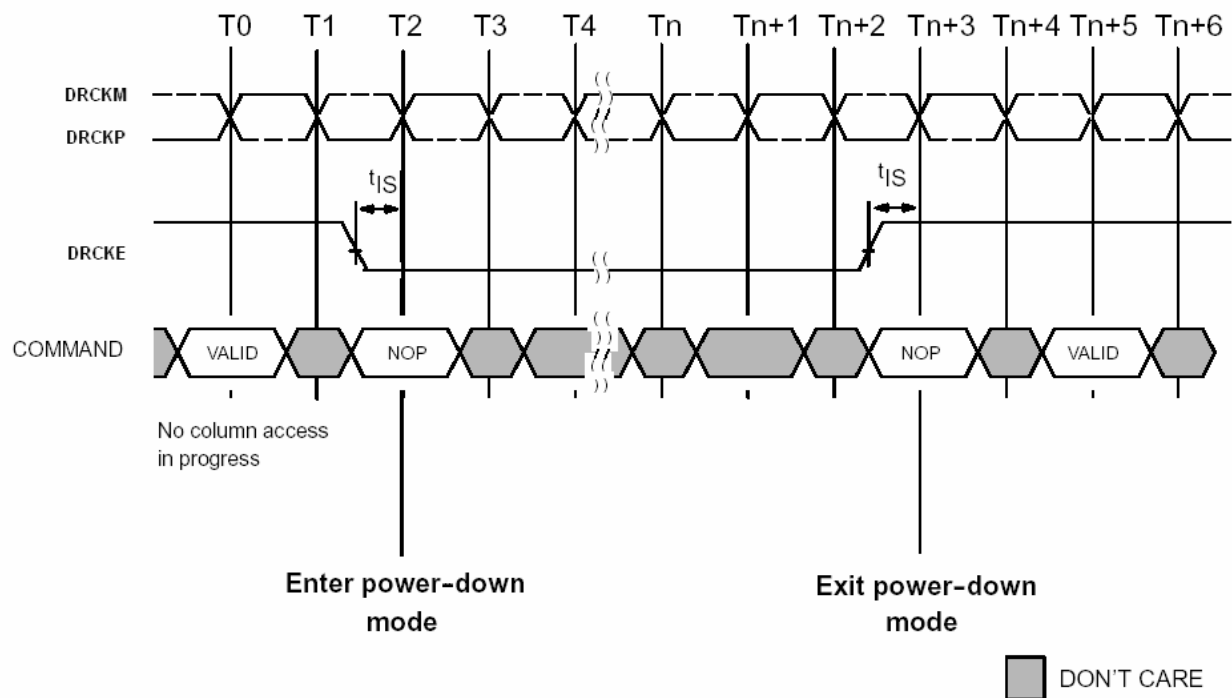
Figure 15-6 Power-Down Command
