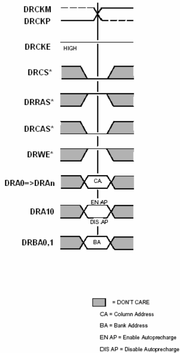
Figure 15-1 Read Command
