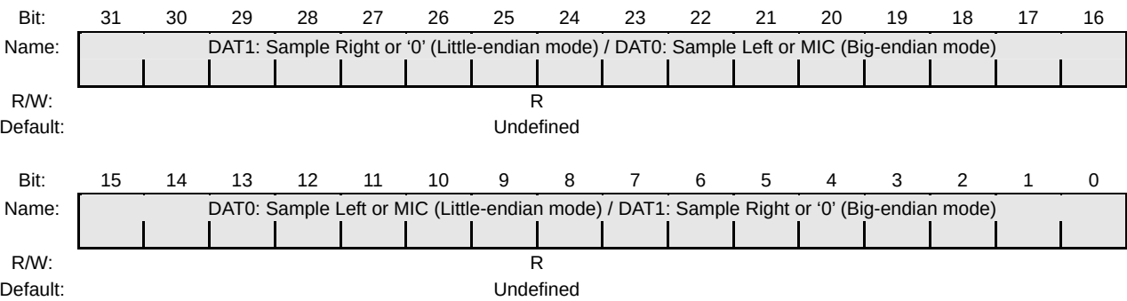
Figure 24-23 ACAUDIDAT Register
