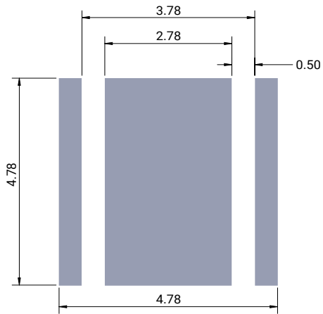
Recommended PCB Footprint
