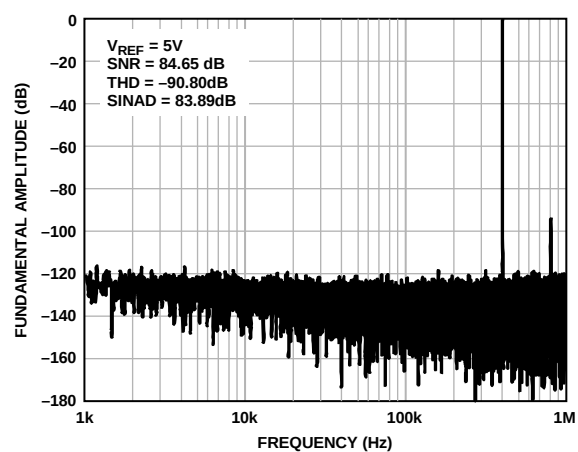
Figure 16. 400 kHz, -0.5 dBFS Input Tone FFT, Wide View
