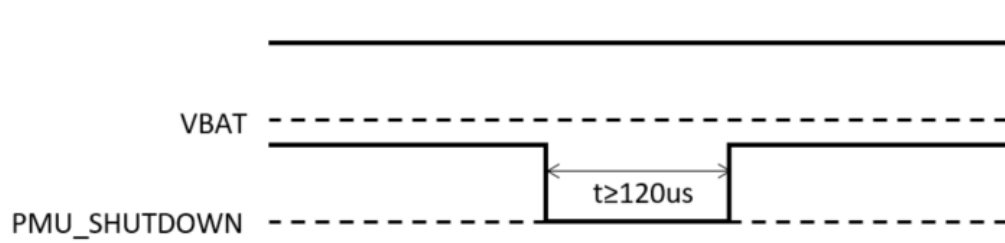
Figure 5.3 Power Sequence Diagram – Power Up
