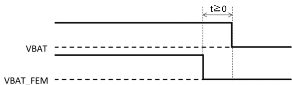
Figure 5.2 Power Sequence Diagram – Power Up
