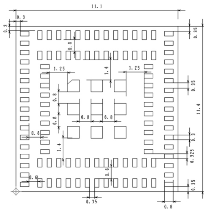
Figure 7.1 Recommended PCB Landing Pattern
