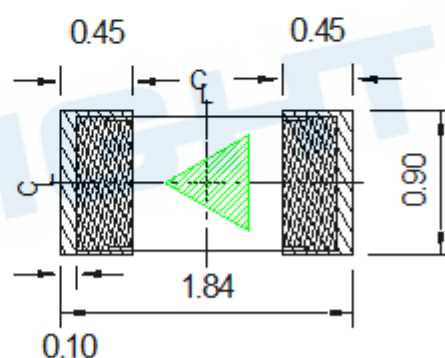
Recommend Soldering pad
