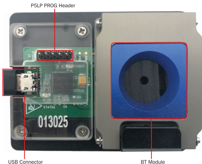
Figure 1: CYBLE-013025-PROG Top View
