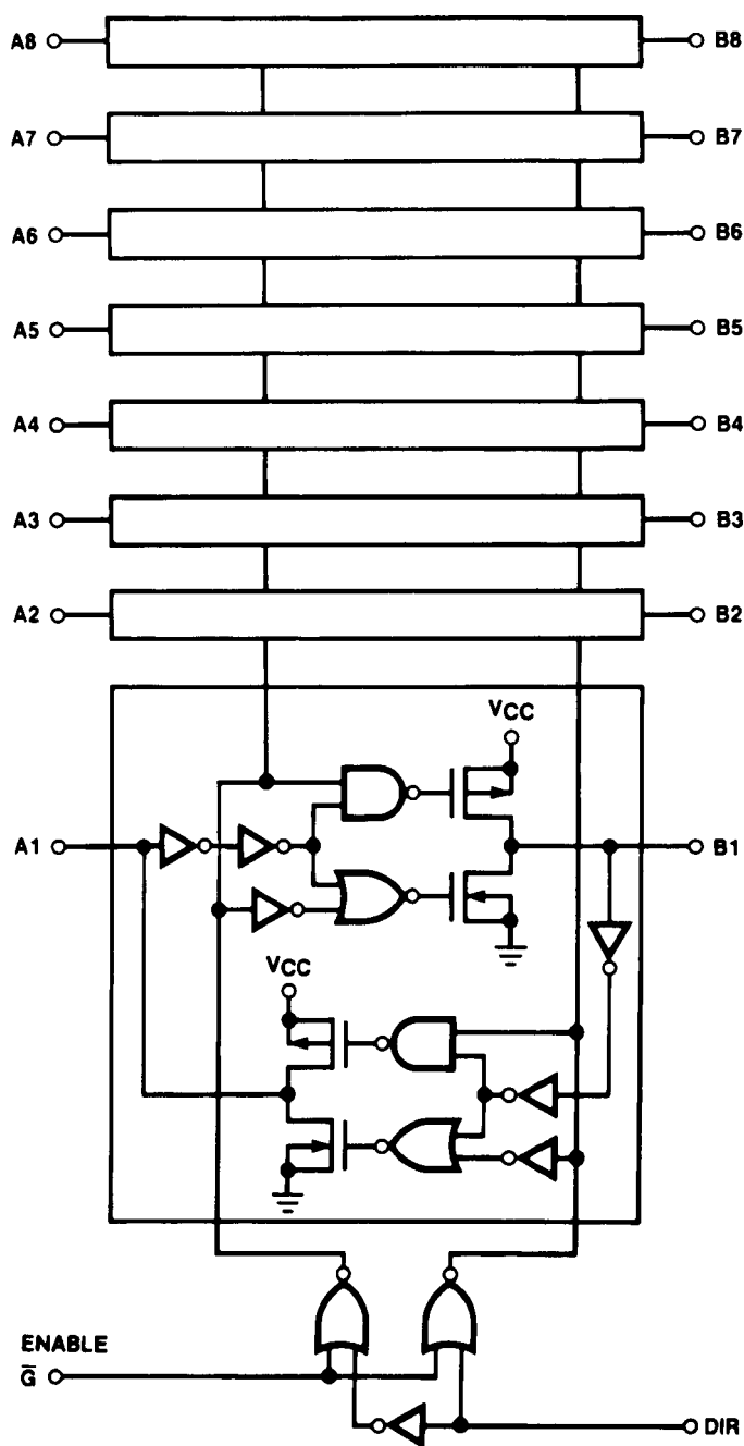
Figure 1. Logic Diagram
