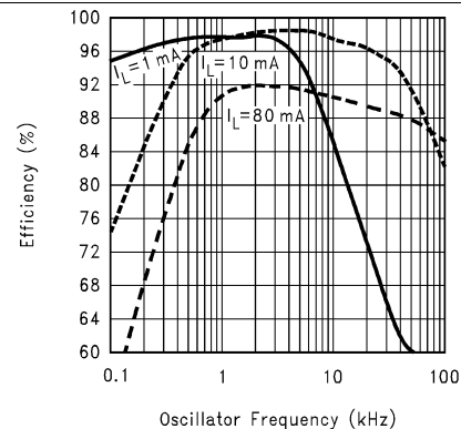
Figure 23. Efficiency vs Oscillator Frequency
