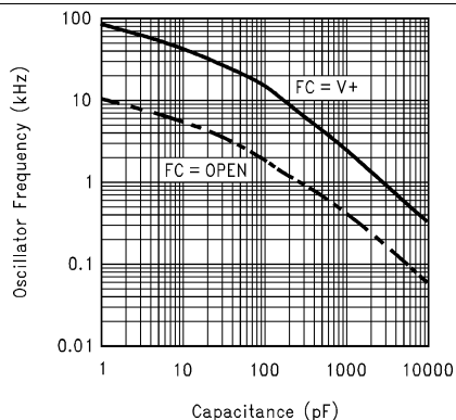
Figure 7. Oscillator Frequency vs External Capacitance
