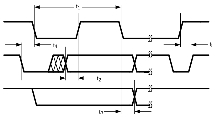
Figure 2. I 2 C Timing
