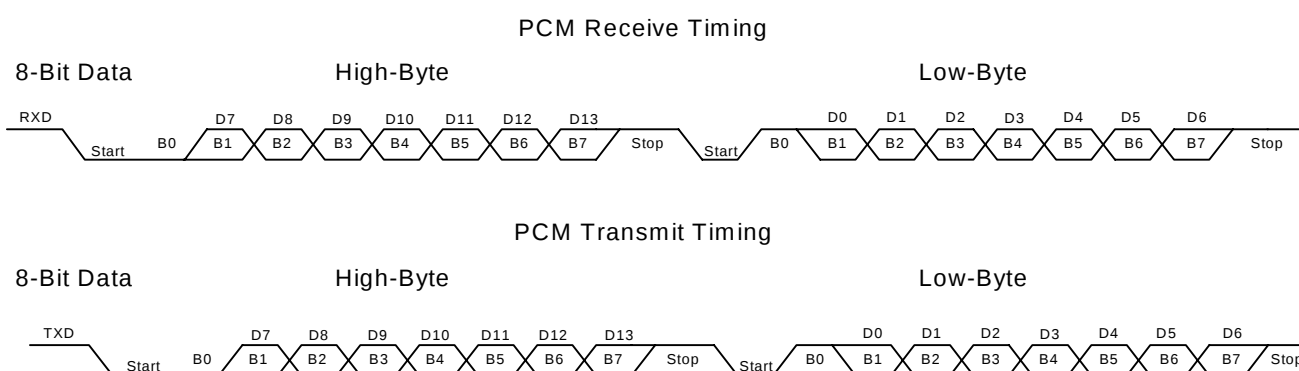
Figure 9. PCM Timing
