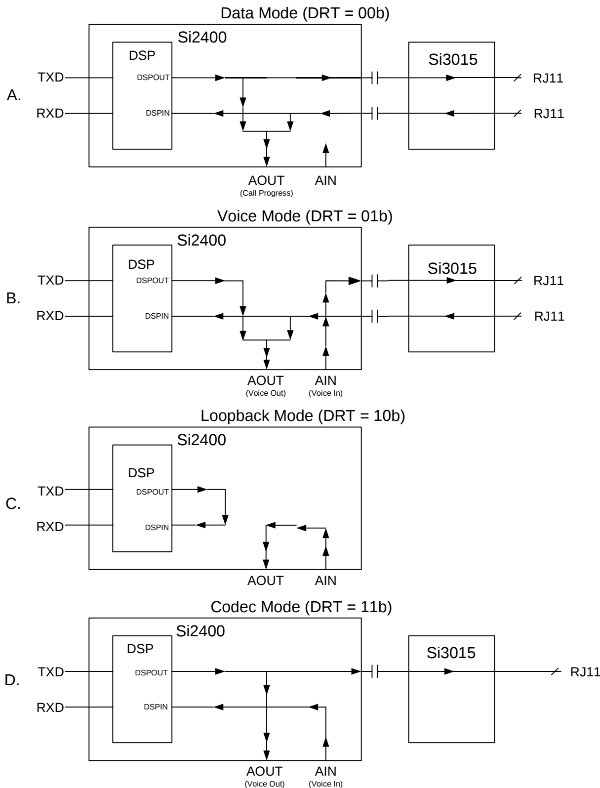
Figure 10. Signal Routing
