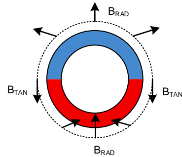
Figure 23: Side-Shaft Field
