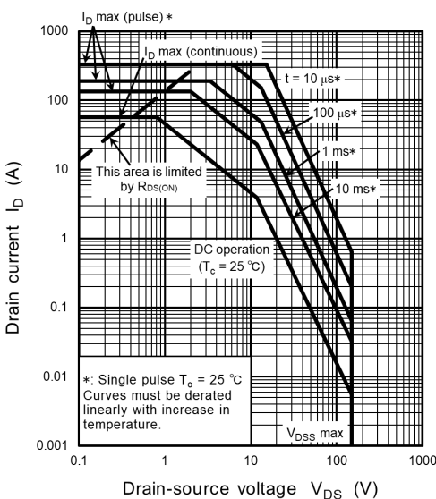
Fig. 8.15 Safe Operating Area (Guaranteed Maximum)
