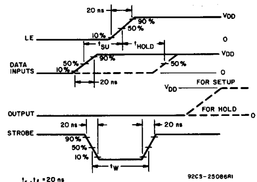
Fig. 14 - Dynamic waveforms.
