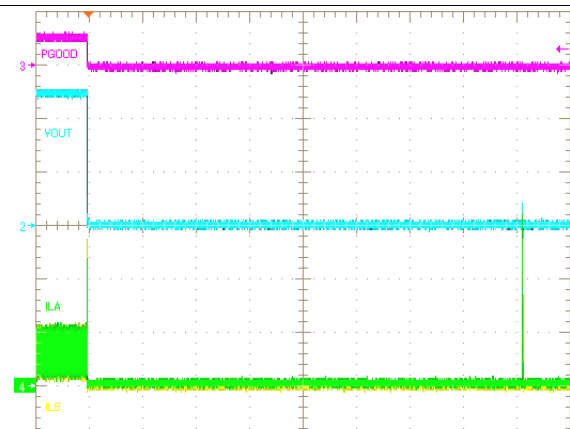
Figure 34. Shutdown Through VIN
