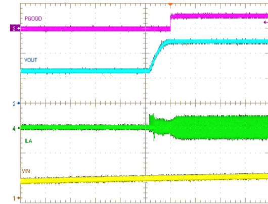
Figure 32. Pre-biased Startup Through VIN
