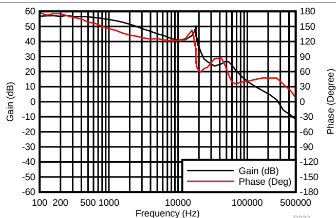
Figure 52. Loop Response
