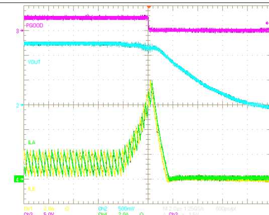
Figure 33. Shutdown Through VIN
