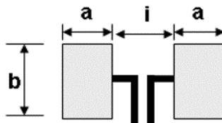
Recommended Solder Pad
