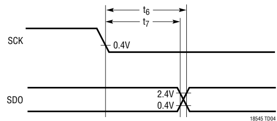
t_6 (Delay Time, \overline{SCK} to SDO Valid) t_7 (Time from Previous Data Remains Valid After \overline{SCK} )
