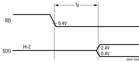
t_8 (SDO Valid After \overline{RD} )
