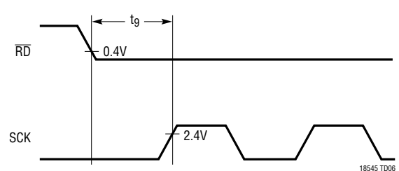
t_9 ( \overline{RD} to SCK Setup Time)
