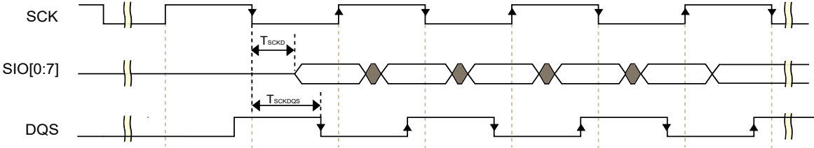
Figure 18. FlexSPI input timing in DDR mode where FlexSPI_MCR0[RXCLKSRC] = 0x3 (case B1)
