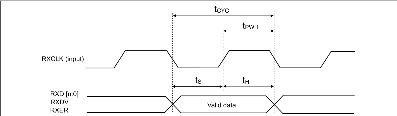
Figure 47. MII Receive Timing
