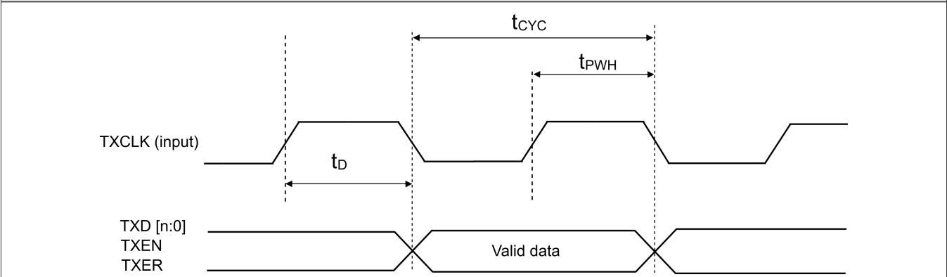
Figure 48. MII Transmit Timing
