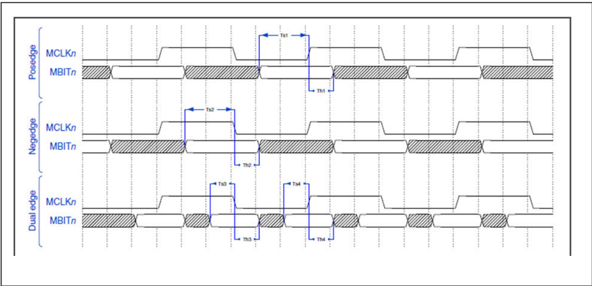
Figure 40. SINC timing
