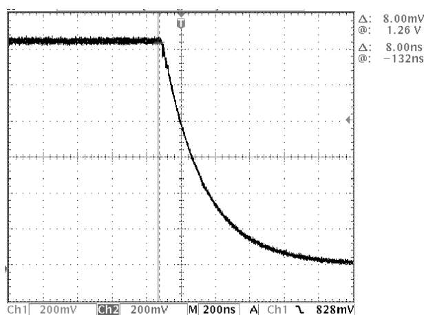
FIGURE 11. DLY_VTH AND DLY_ICHG TIMING MISMATCH
