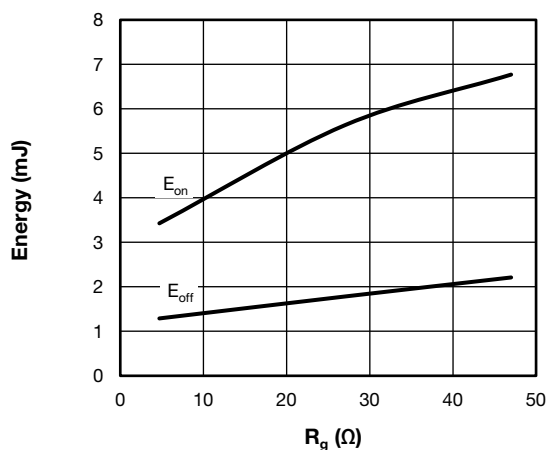
Fig. 11 - Typical IGBT Energy Losses vs. R_g T_J = 125^\circ\text{C} , I_C = 50\text{ A} , V_{CC} = 600\text{ V} , V_{GE} = 15\text{ V} , L = 500\text{ }\mu\text{H}
