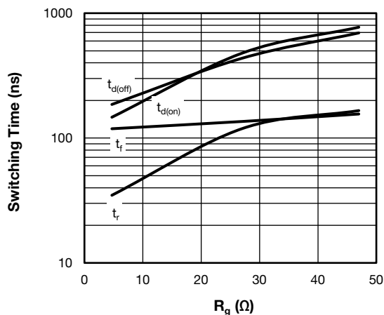
Fig. 12 - Typical IGBT Switching Time vs. R_g T_J = 125^\circ\text{C} , I_C = 50\text{ A} , V_{CC} = 600\text{ V} , V_{GE} = 15\text{ V} , L = 500\text{ }\mu\text{H}
