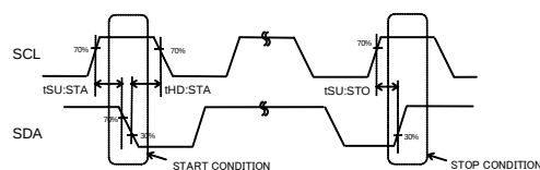
Figure 2-(b). Start-Stop Bit Timing
