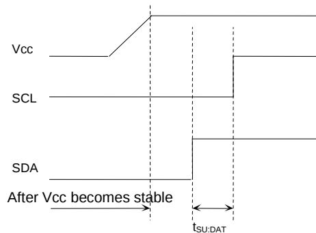
Figure 53. When SCL='L' and SDA='L'
