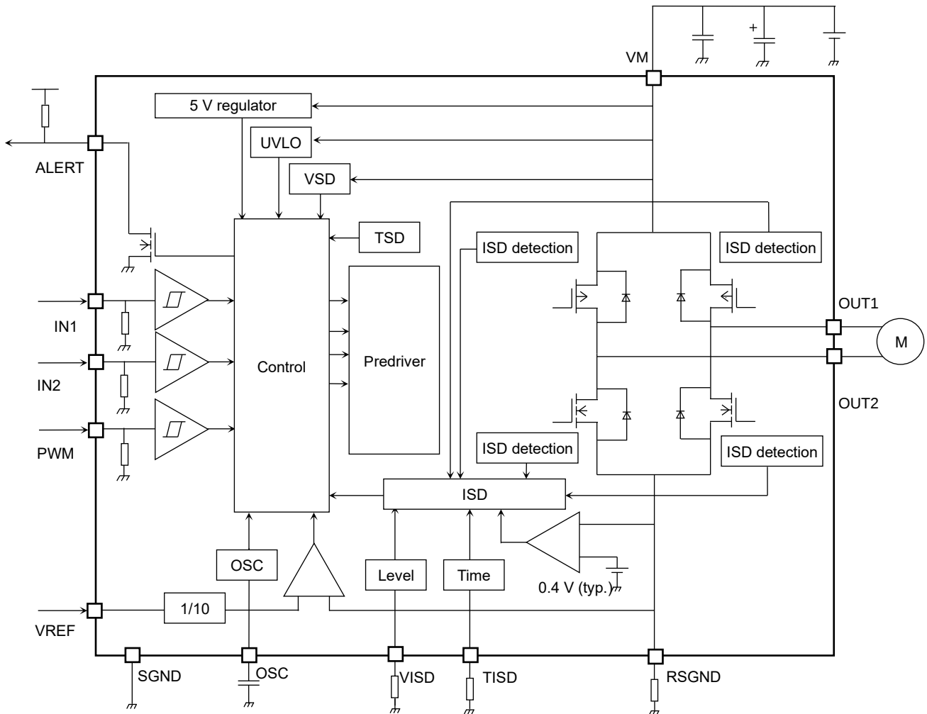
Figure 3 Block Diagram
