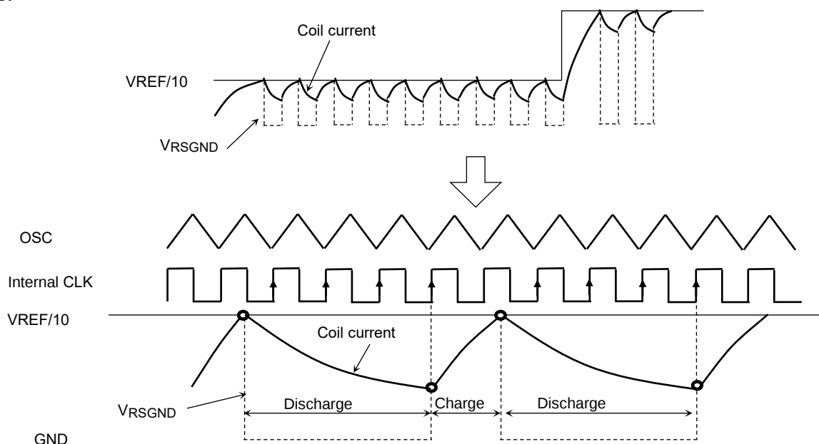
Figure 13.9.2 Constant-current Chopping
