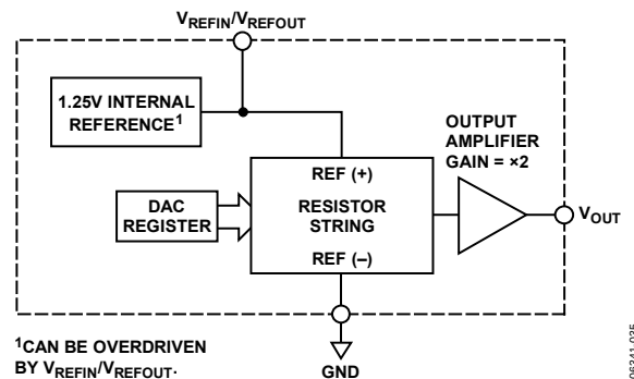
Figure 57. Internal Configuration When Using the Internal Reference
