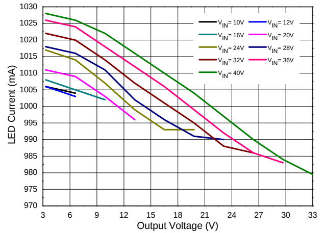
LED Current vs. Output Voltage (R S =0.1Ω, L=68μH)
