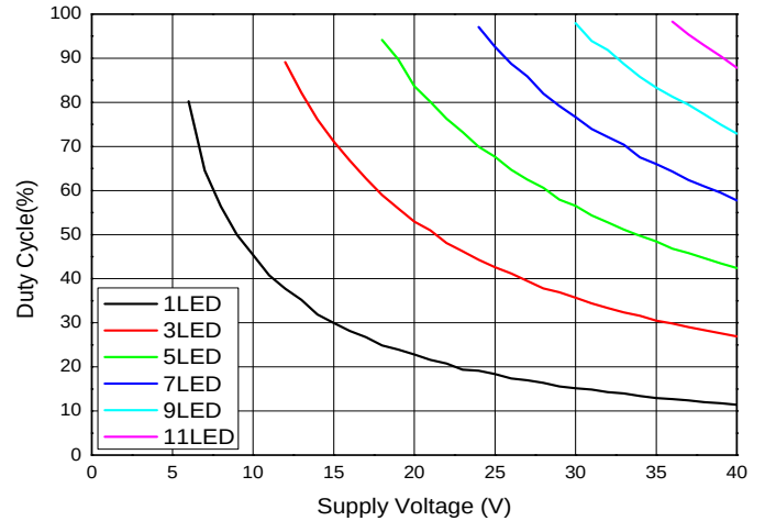
Switching Duty Cycle vs. Supply Voltage (R S =0.067Ω, L=68μH)
