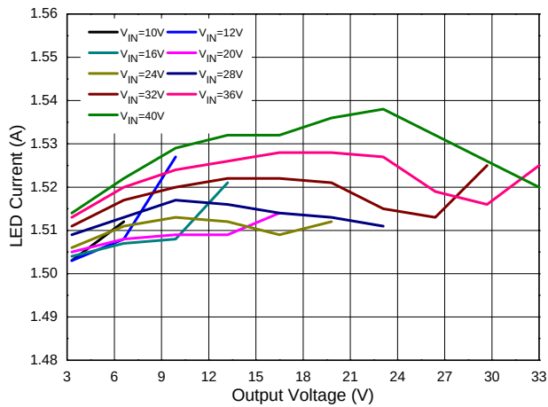
LED Current vs. Output Voltage (R S =0.067Ω, L=47μH)
