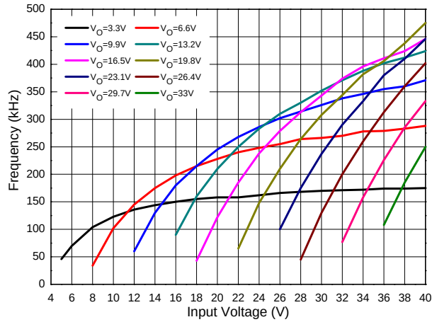
Operating Frequency vs. Input Voltage (R S =0.067Ω, L=47μH)
