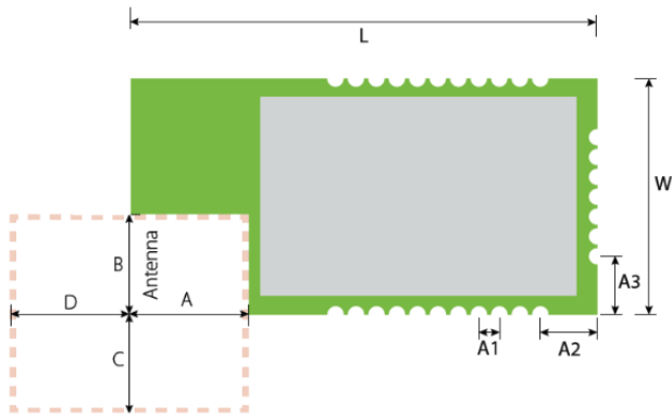
Figure 4. Physical Dimensions
