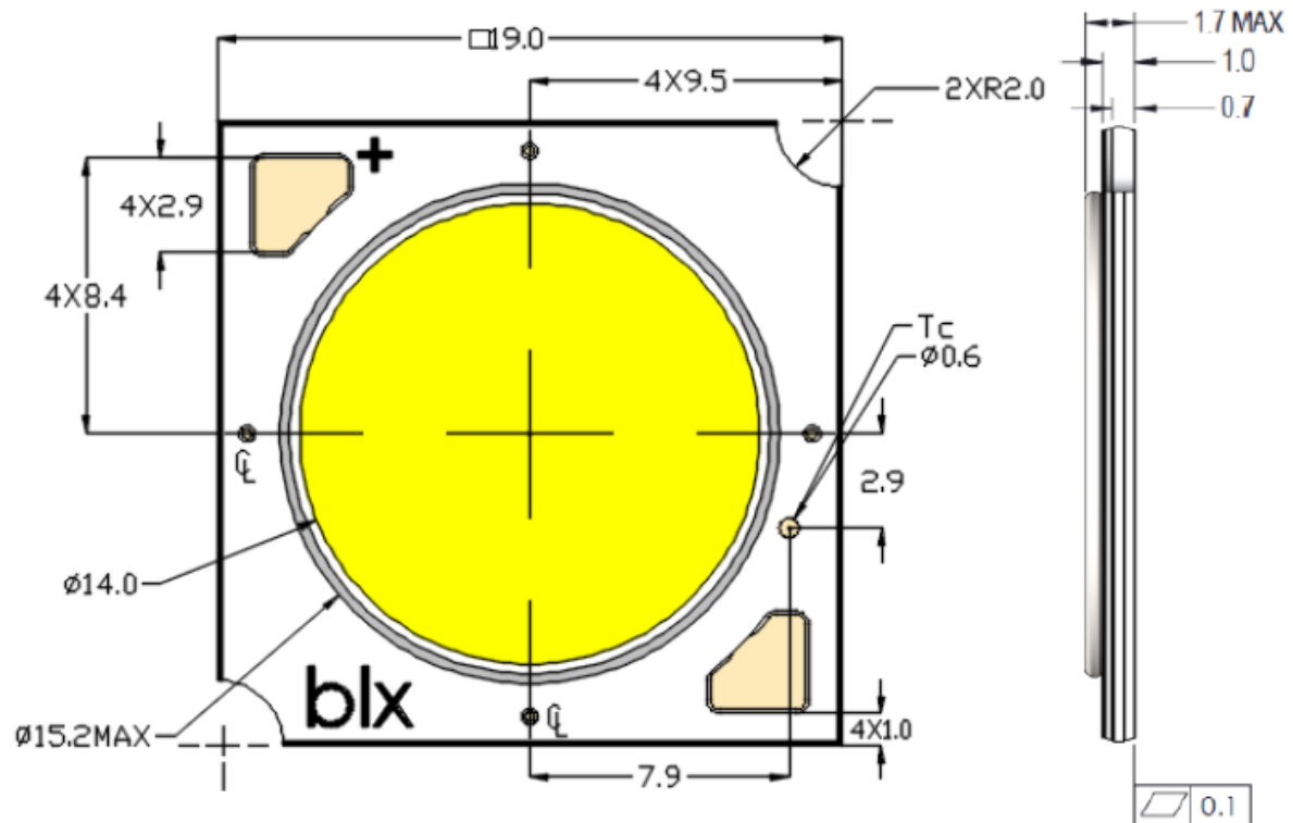
Figure 17: Drawing for V13 LED Array
