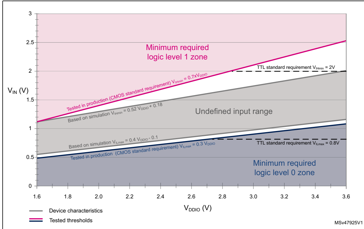
Figure 18. V_{IL}/V_{IH} for all I/Os except BOOT0
