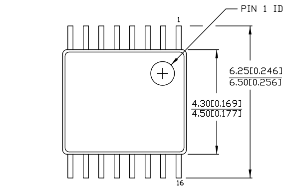
Figure 10. 16-pin TSSOP (4.40 mm Body) Z16.173/ZZ16.173, 51-85091
