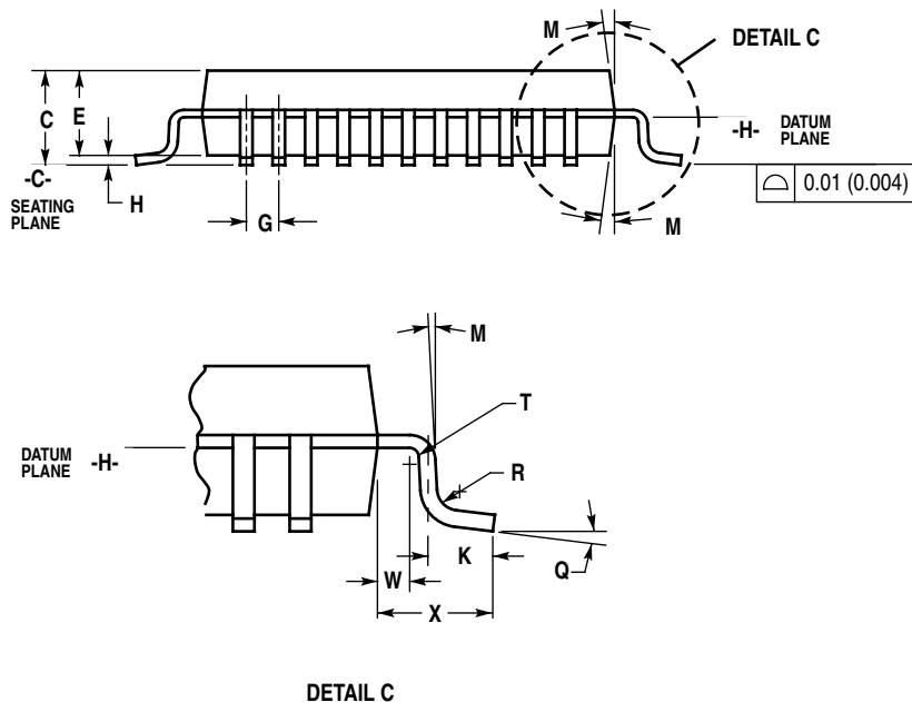
DETAIL C
