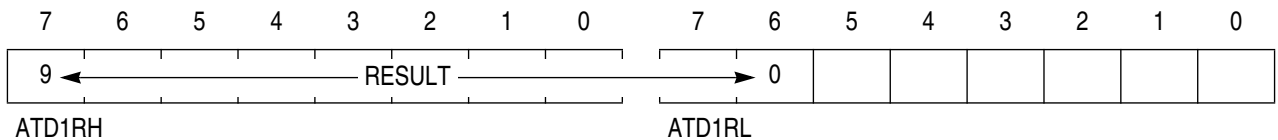
Figure 14-6. Left-Justified Mode
