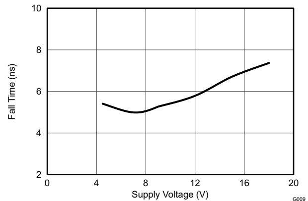
Figure 5-18. Fall Time vs Supply Voltage
