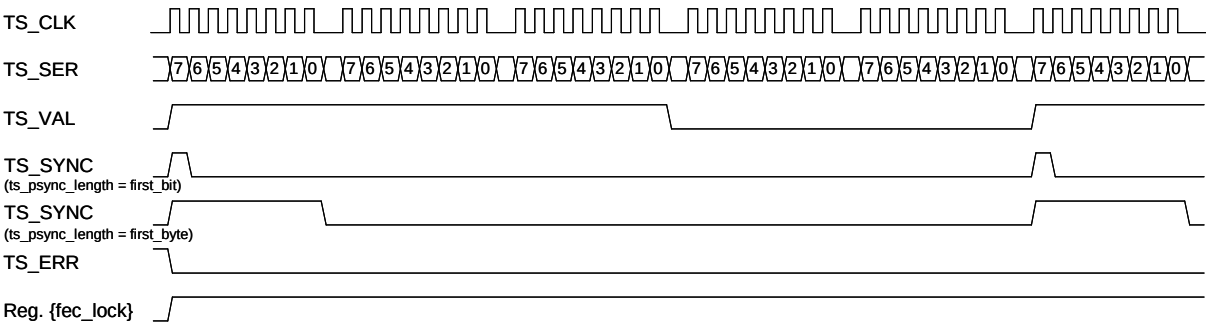
Figure 17. Gapped TS Serial Mode with Rising Active Clock Edge, Enabled Parity Bytes, and Active High Polarities
