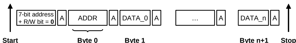
Figure 22. I 2 C Write Command Sequence in 8-Bit Addressing Mode
