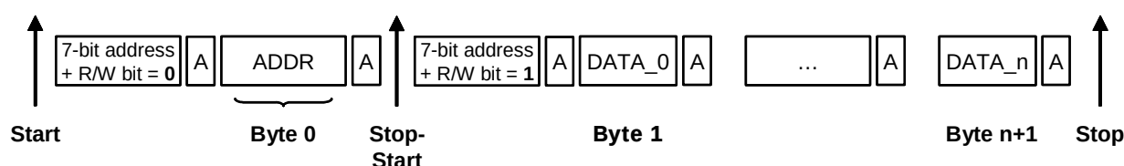
Figure 23. I 2 C Read Command Sequence in 8-Bit Addressing Mode
