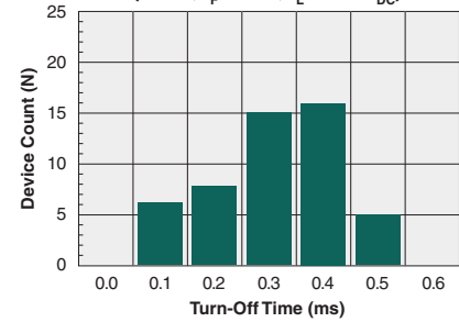
Typical Turn-Off Time (N=50, I_F=8\text{mA} , I_L=85\text{mA}_{DC} )
