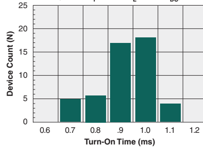
Typical Turn-On Time (N=50, I_F=8\text{mA} , I_L=85\text{mA}_{DC} )
