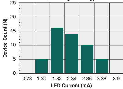
Typical I_F for Switch Operation (N=50, I_L=85\text{mA}_{DC} )
