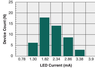
Typical I_F for Switch Dropout (N=50, I_L=85\text{mA}_{DC} )
