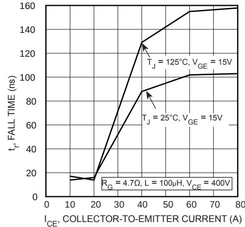
FIGURE 12, Current Fall Time vs Collector Current
