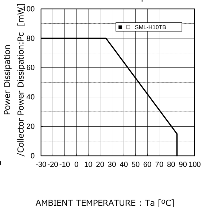
Fig.4 Power Dissipation/Collector Power Dissipation - Ambient Temperature
