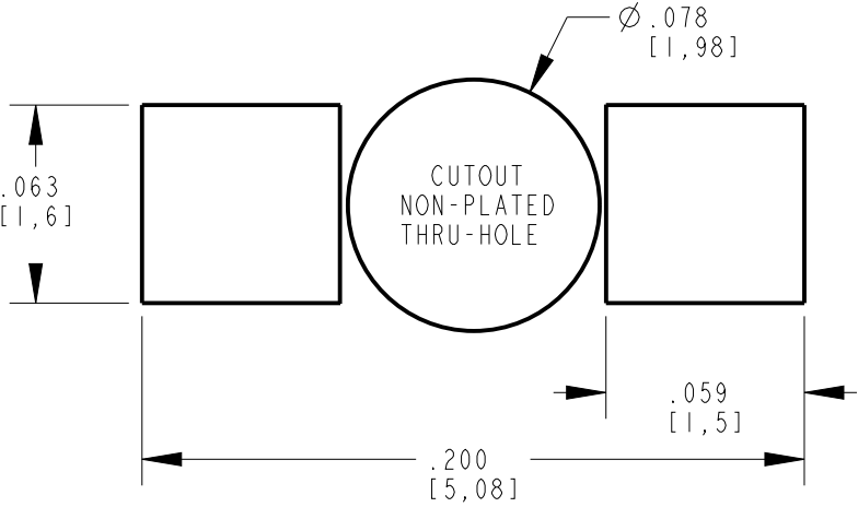
PRINTED CIRCUIT BOARD ATTACHMENT PAD
