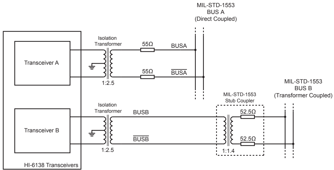
Figure 27. Bus Connection Example using HI-6138
