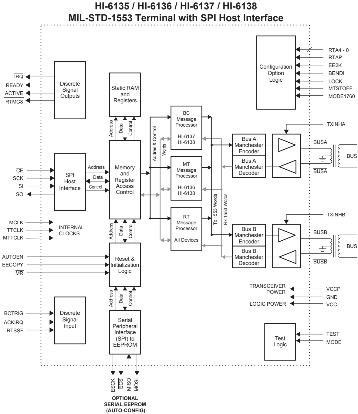
Figure 1. Block Diagram
