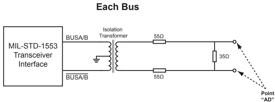
Figure 28. MIL-STD-1553 Direct Coupled Test Circuits
