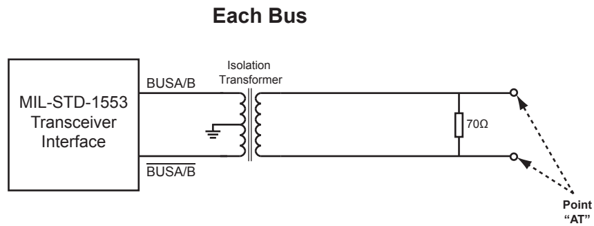
Figure 29. MIL-STD-1553 Transformer Coupled Test Circuits
