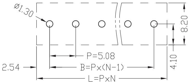
PCB LAYOUT
