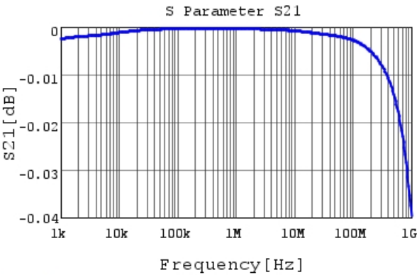
ECASD40G157M016K00 S21 DCOV, 25degC
