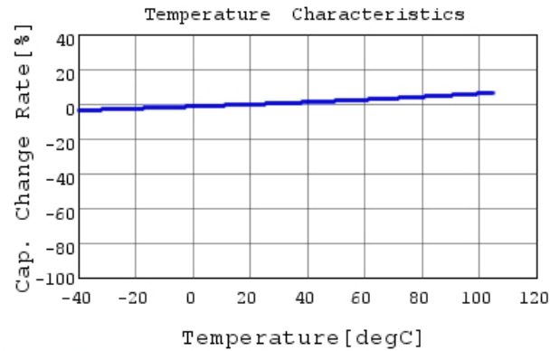
ECASD40G157M016K00 C-Temp. capchange, DCOV,
