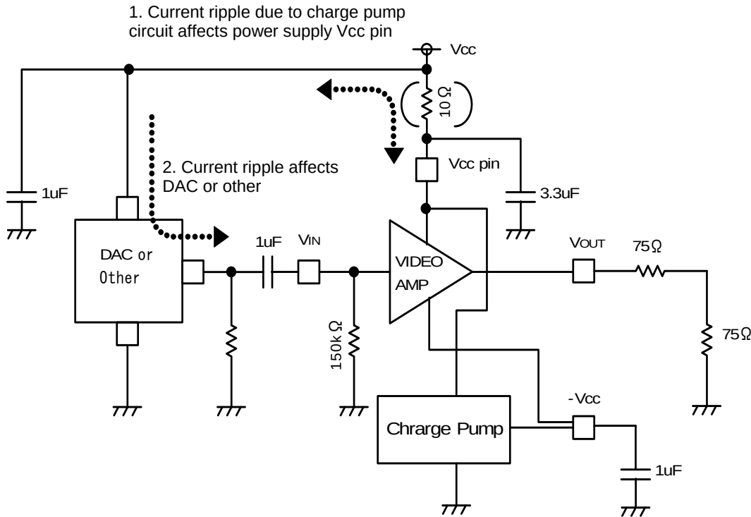
Fig.12 Effects of Charge Pump Circuit Current Ripple on External Circuit
