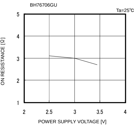
Fig. 57 Output Pin Shunt Switch On Resistance vs Supply Voltage
