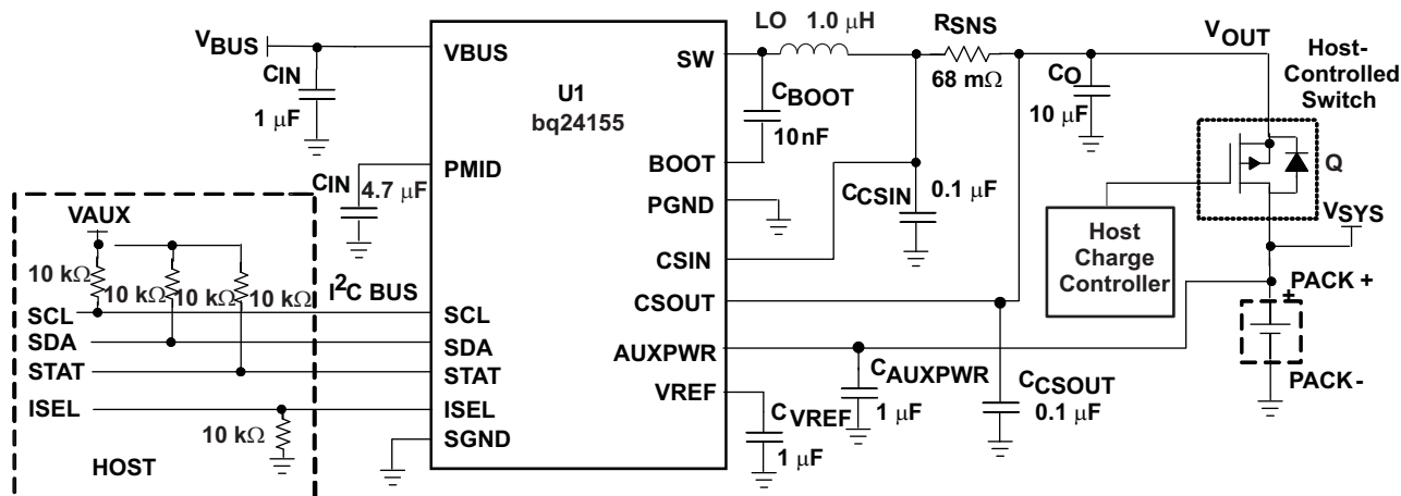
Figure 2. I²C Controlled 1-Cell Pre-Regulator Application
