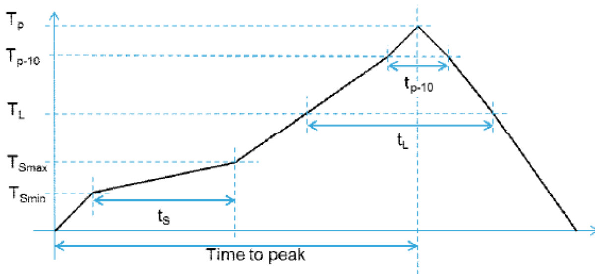
Figure 34. Solder profile
