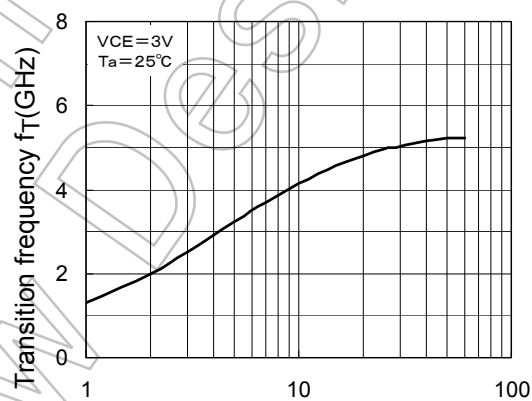
f_T-I_C
