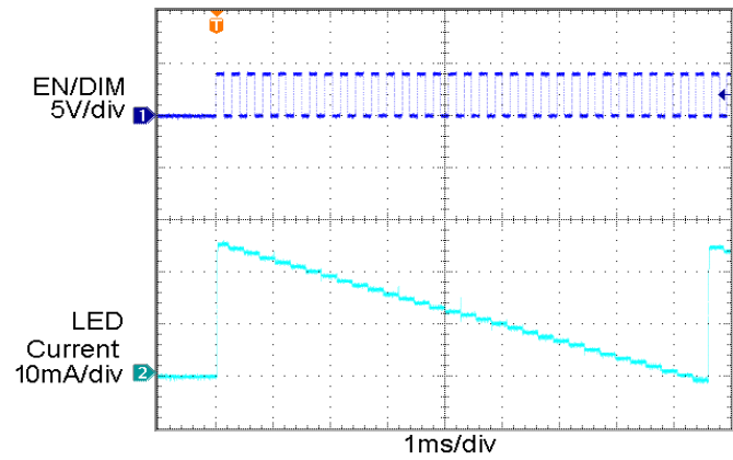
Figure 14. Dimming Levels
